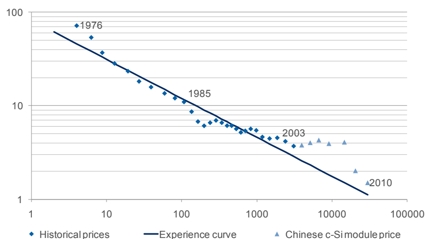
Figure 10: Solar module experience curve, 1975-2020
